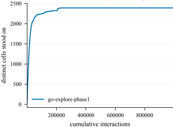
States discovered -- TopMobius-50@4001
