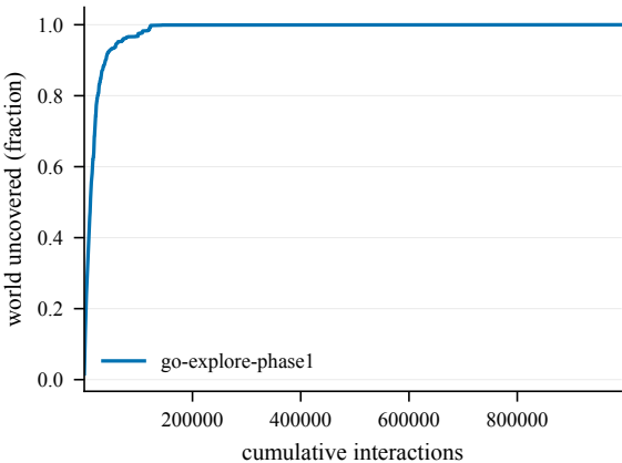
Cumulative coverage -- TopMobius-50@4002
