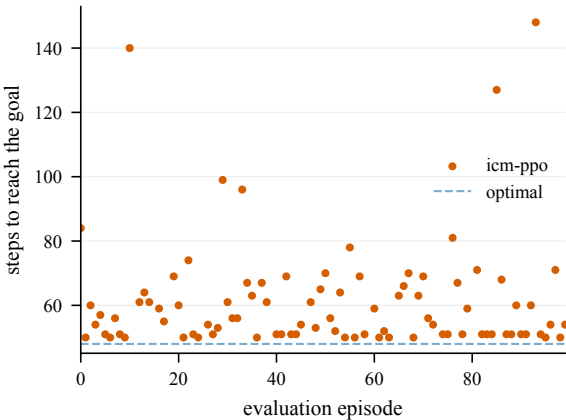
Steps to goal (eval) -- TopMobius-50@4002
