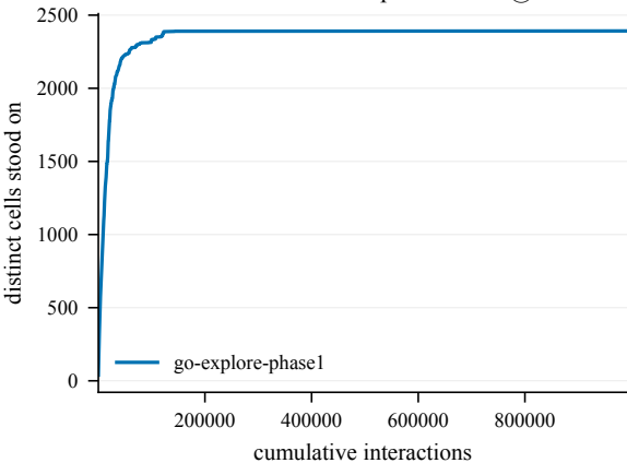
States discovered -- TopMobius-50@4002
