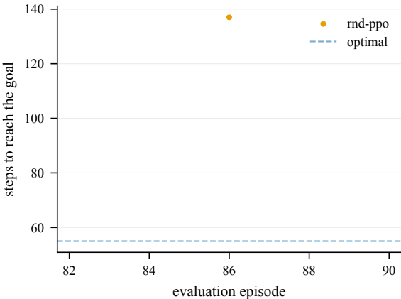
Steps to goal (eval) -- TopPlane-50@4000
