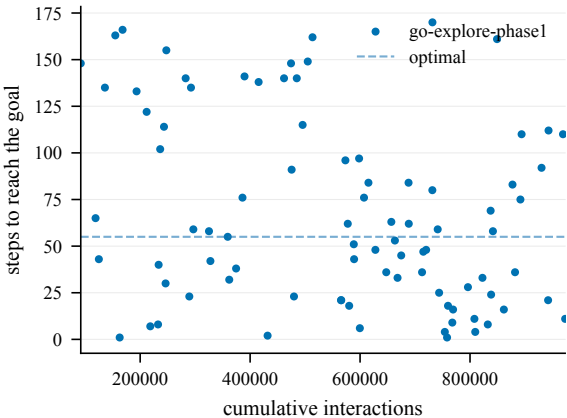
Steps to goal (train) -- TopPlane-50@4000
