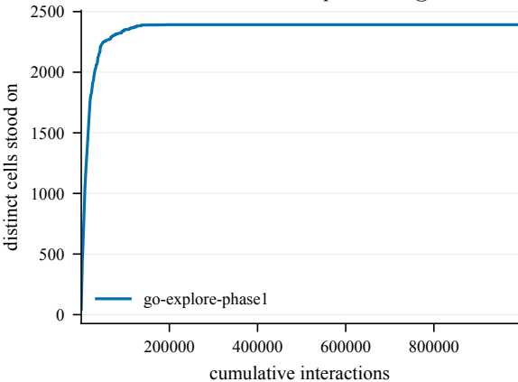
States discovered -- TopPlane-50@4000
