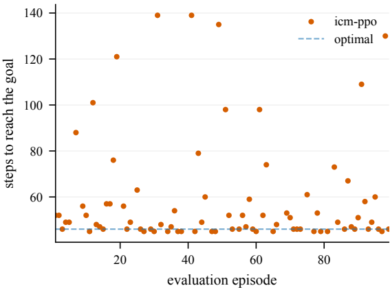
Steps to goal (eval) -- TopPlane-50@4001
