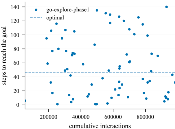
Steps to goal (train) -- TopPlane-50@4001
