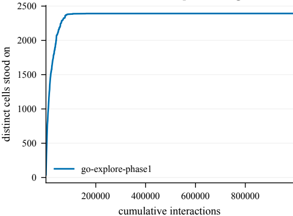
States discovered -- TopPlane-50@4002
