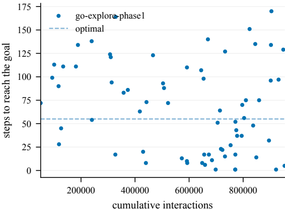
Steps to goal (train) -- TopRP2-50@4000
