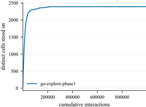
States discovered -- TopRP2-50@4000
