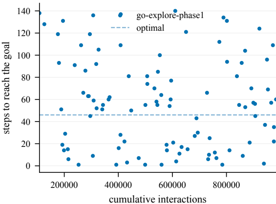
Steps to goal (train) -- TopRP2-50@4001
