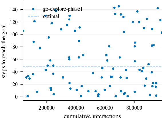
Steps to goal (train) -- TopRP2-50@4002
