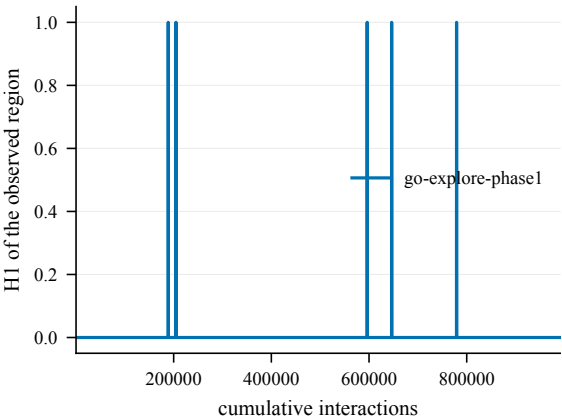
Discovered topology -- TopTorus-50@4000
