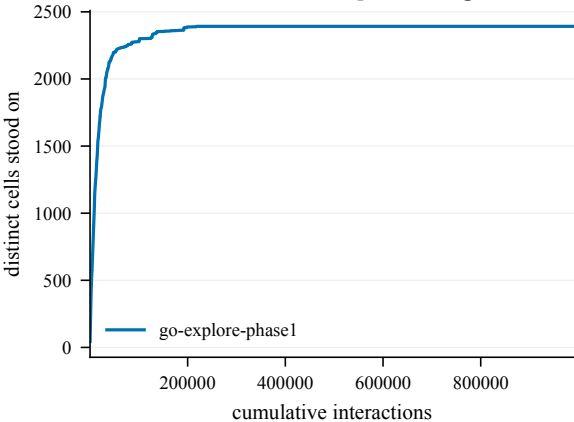
States discovered -- TopTorus-50@4000
