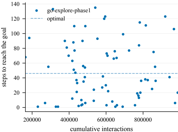
Steps to goal (train) -- TopTorus-50@4001
