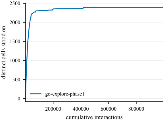
States discovered -- TopTorus-50@4001
