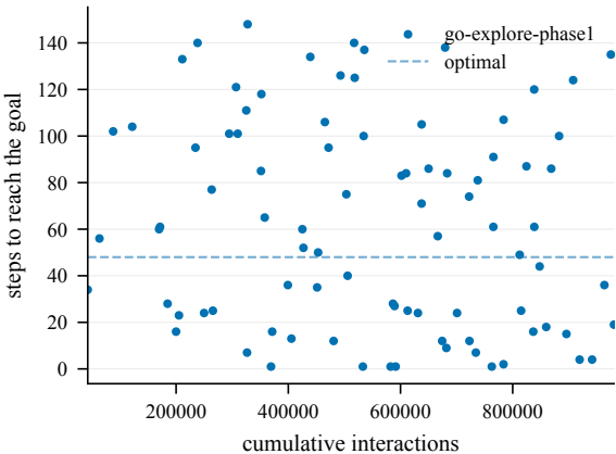
Steps to goal (train) -- TopTorus-50@4002
