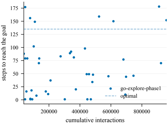
Steps to goal (train) -- EpicChase12-150@11
