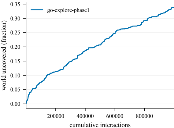
Cumulative coverage -- EpicChase12-150@14
