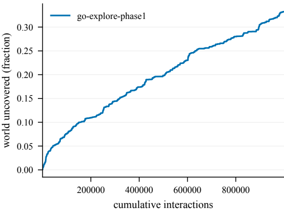
Cumulative coverage -- EpicChase12-150@22
