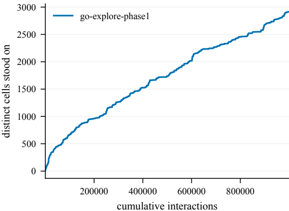
States discovered -- EpicChase12-150@22
