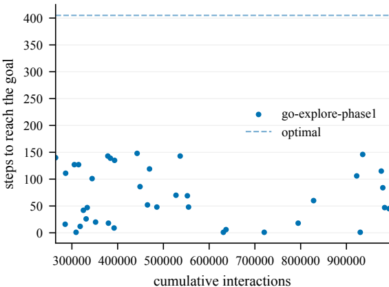
Steps to goal (train) -- EpicChase12-150@23
