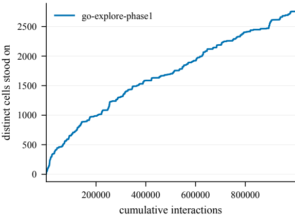
States discovered -- EpicChase12-150@26
