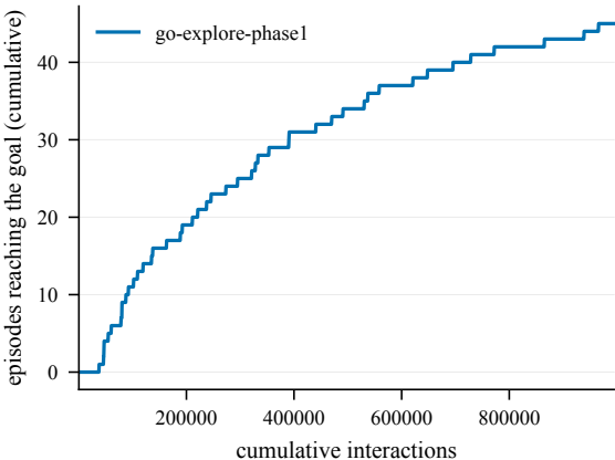
Goal reached -- EpicChase12-150@27
