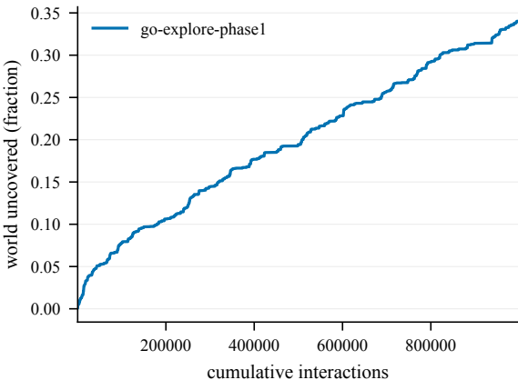
Cumulative coverage -- EpicChase12-150@29
