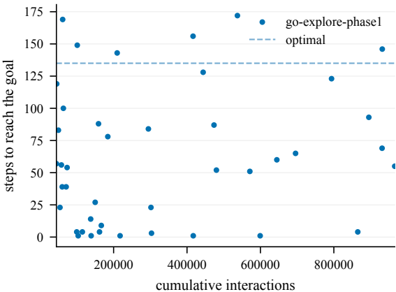
Steps to goal (train) -- EpicChase6-110@11
