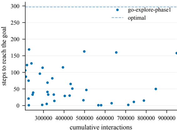
Steps to goal (train) -- EpicChase6-110@13
