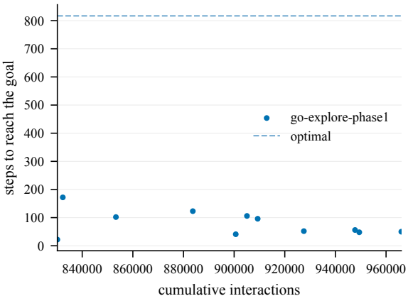
Steps to goal (train) -- EpicChase6-110@14
