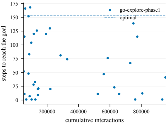
Steps to goal (train) -- EpicChase6-110@15
