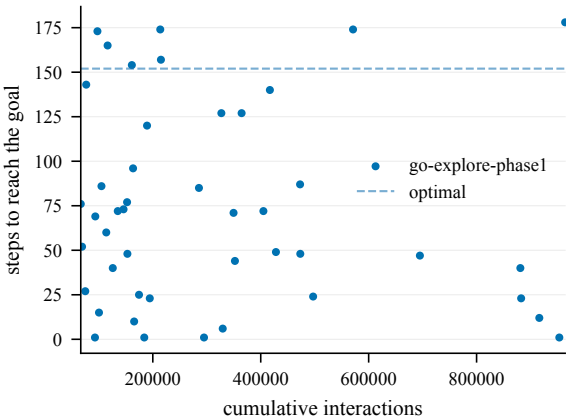
Steps to goal (train) -- EpicChase6-110@18
