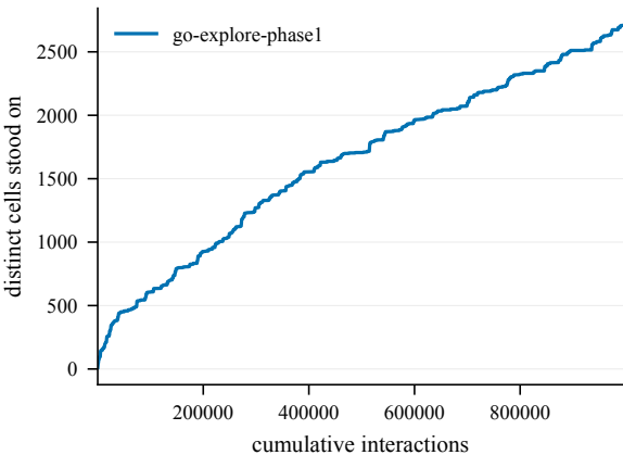
States discovered -- EpicChase6-110@18
