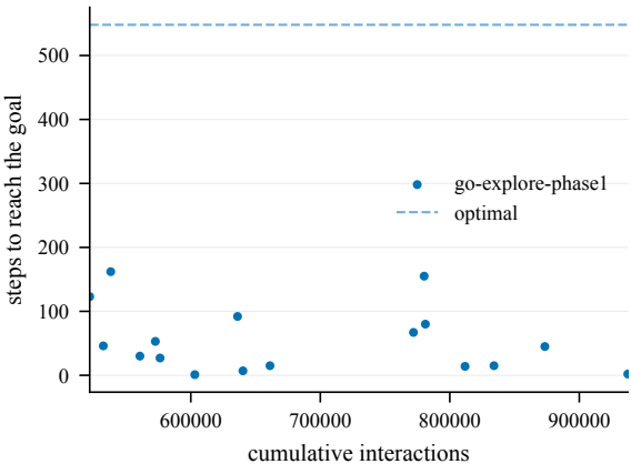
Steps to goal (train) -- EpicChase6-110@20
