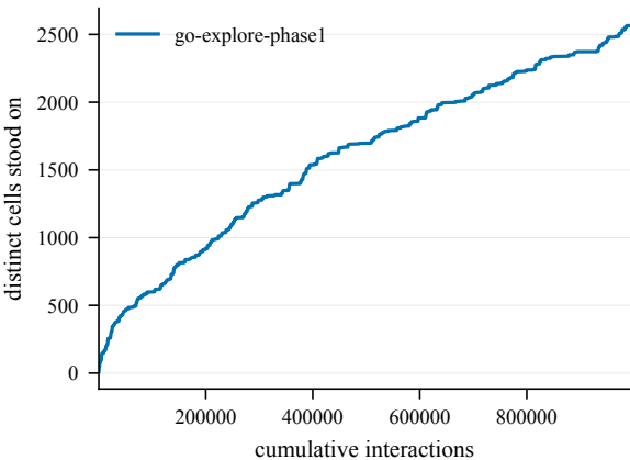
States discovered -- EpicChase6-110@21
