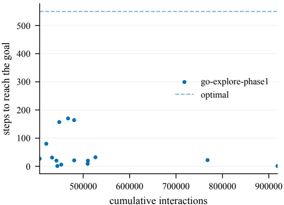
Steps to goal (train) -- EpicChase6-110@22
