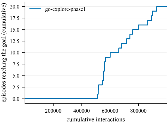
Goal reached -- EpicChase6-110@24
