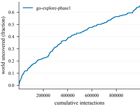
Cumulative coverage -- EpicChase6-110@25
