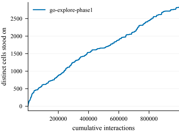
States discovered -- EpicChase6-110@26
