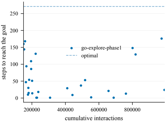
Steps to goal (train) -- EpicChase6-110@27
