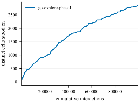
States discovered -- EpicChase6-110@27
