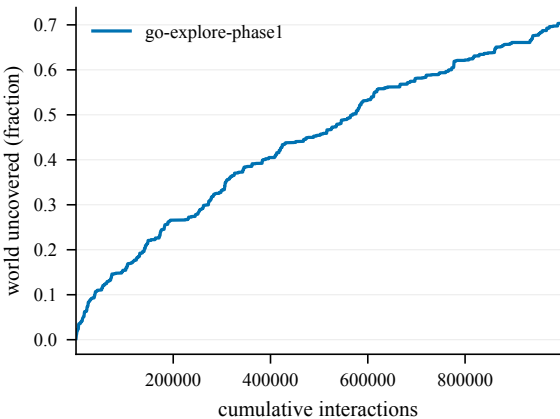
Cumulative coverage -- EpicChase6-110@28
