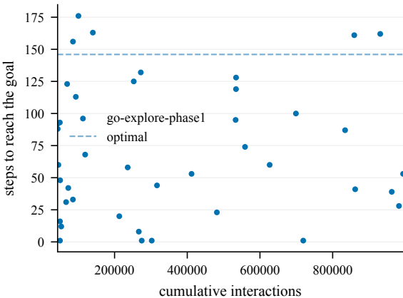
Steps to goal (train) -- EpicChase6-110@28
