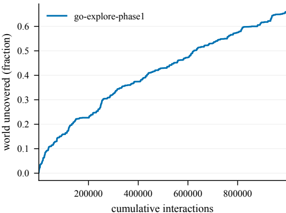
Cumulative coverage -- EpicChase6-110@29
