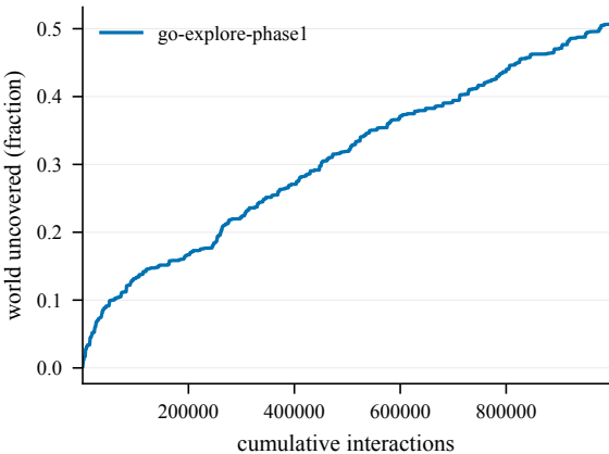
Cumulative coverage -- EpicChase8-120@11
