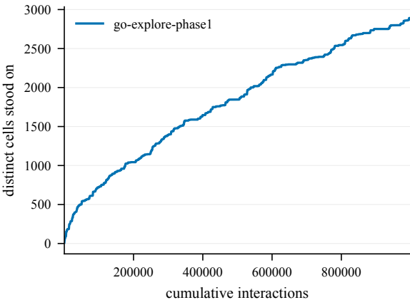
States discovered -- EpicChase8-120@14
