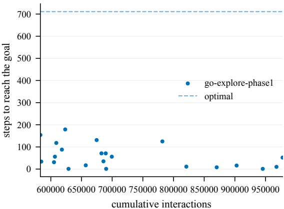
Steps to goal (train) -- EpicChase8-120@15
