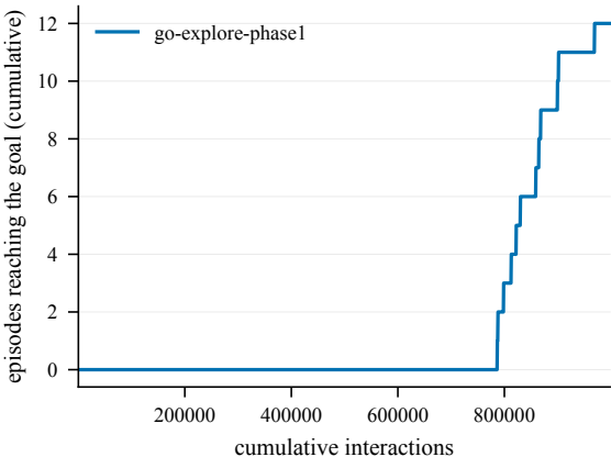
Goal reached -- EpicChase8-120@16
