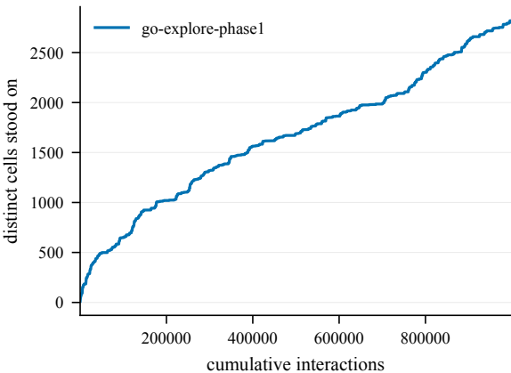
States discovered -- EpicChase8-120@16
