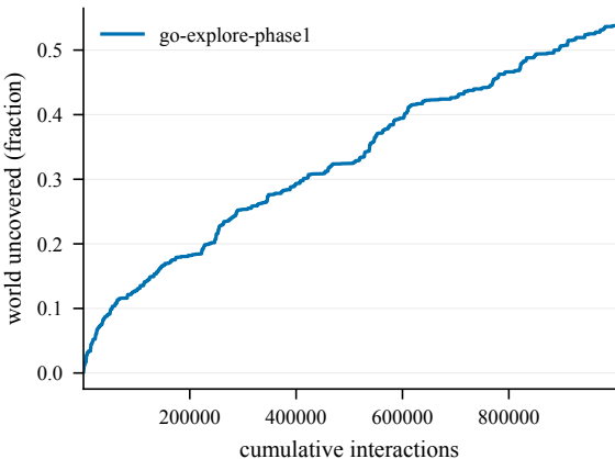
Cumulative coverage -- EpicChase8-120@18
